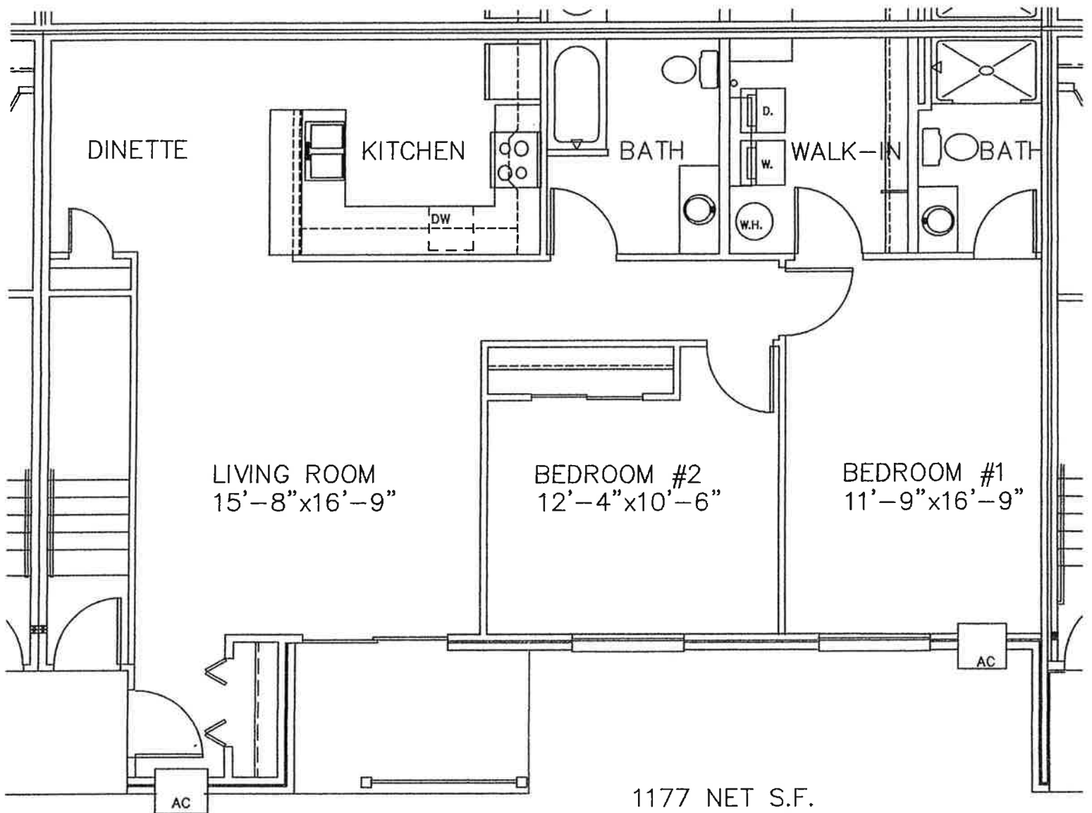
FIRST FLOOR PLAN 12 UNIT STYLE A
