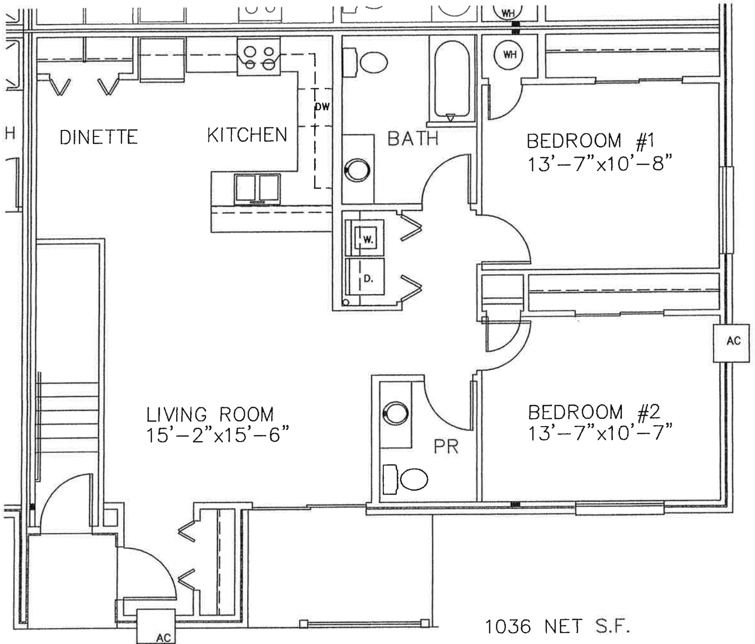
FIRST FLOOR PLAN 12 UNIT STYLE A
